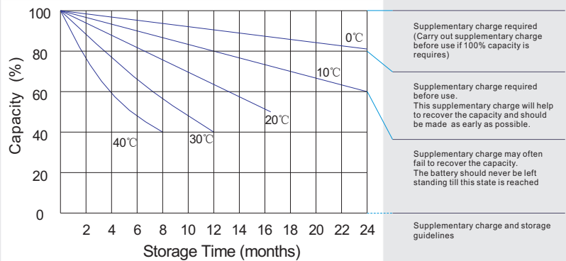
Storage characteristic
