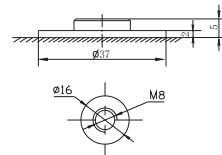
Terminal F5
